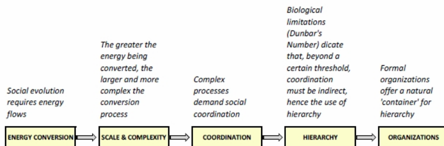
Fig 4. From Energy Conversion to Hierarchical Organization
