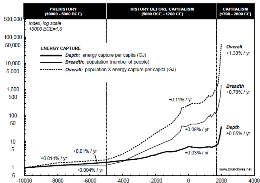
Figure 1: World Energy Capture
