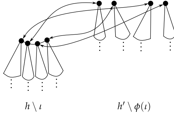
Figure 8: Illustrating Theorem 1 .
